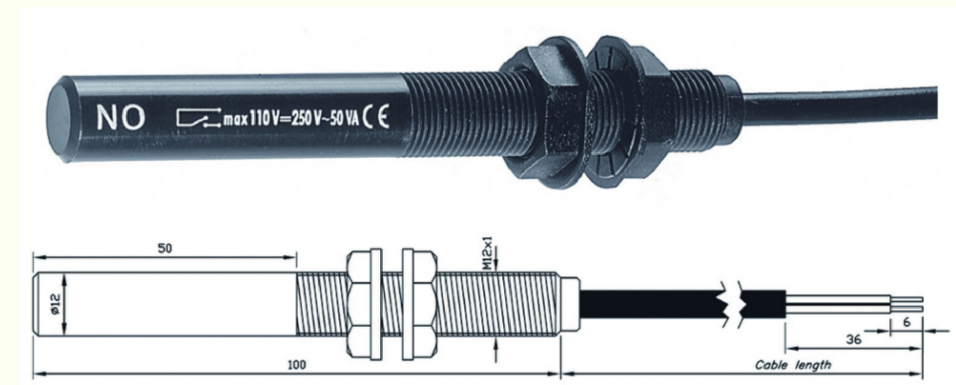
▶ MAGNETIC SENSOR
