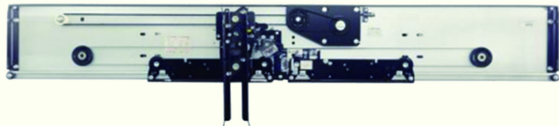
▶ CENTER-OPENING 2 PANELS DOOR OPERATOR
